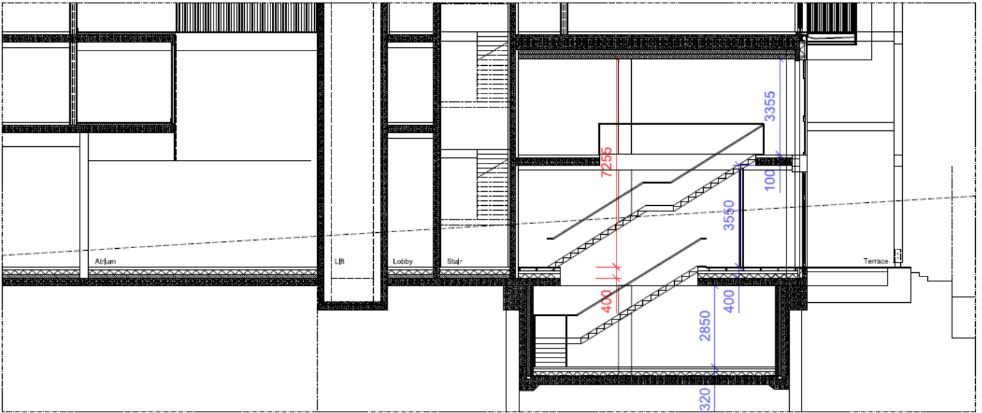
01 Section Through Café Space
