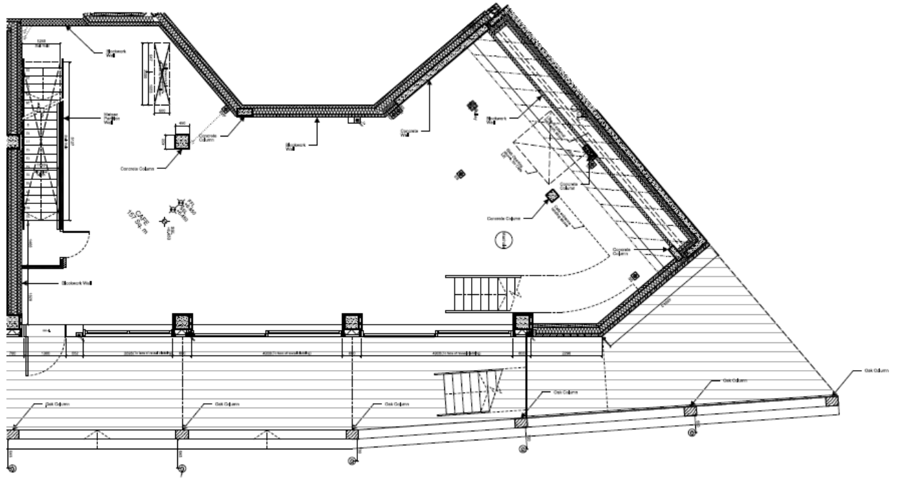
01 Café Space Ground Floor
